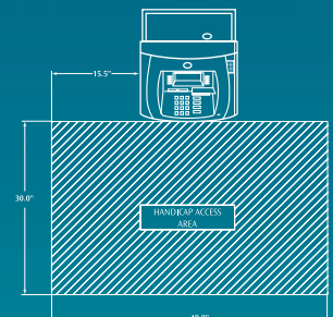
ATM INSTALLATION SPACE REQUIREMENTS FOR ADA COMPLIANCE
